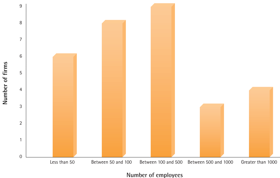
Figure 7: Company Size
